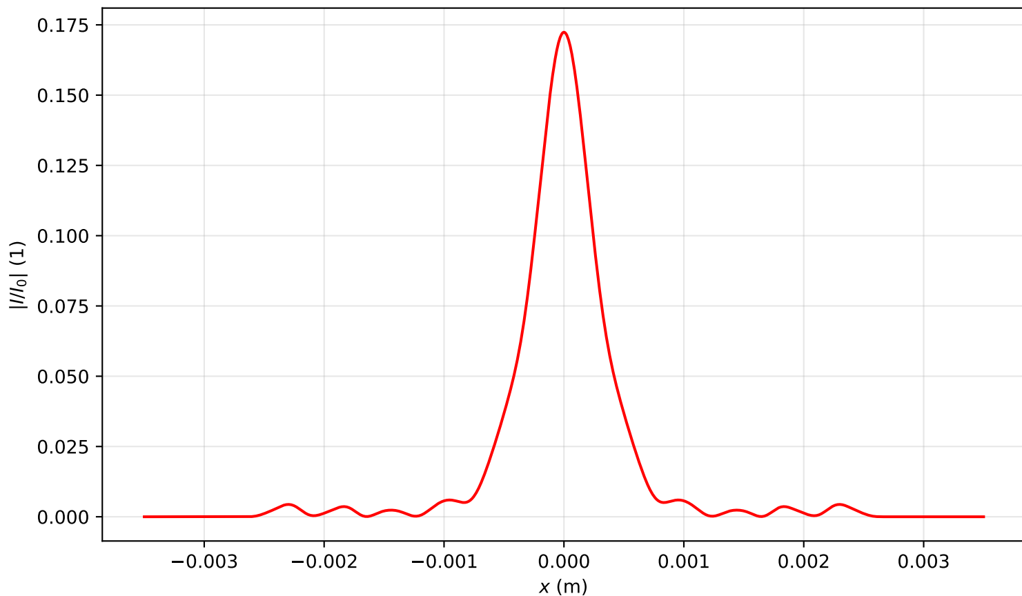
Intensity profile I(x, y = 0, z = 3.184)/I_0 , P_{in}=6.0P_{cr} , artificial time
